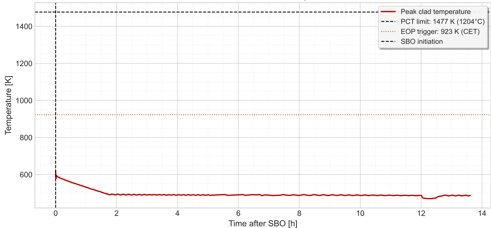
Base Case - Peak Clad Temperature
